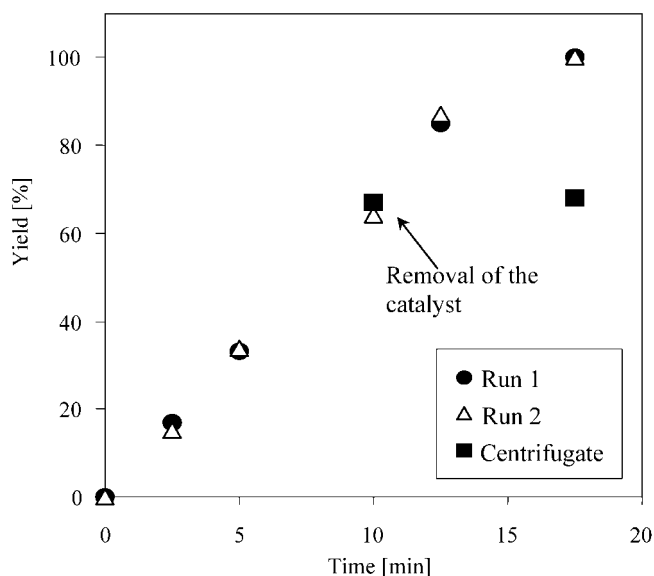
Figure 1. Filtrate test for the bromoethoxylation of DHP in ethanol. Reaction conditions of Table 2.
